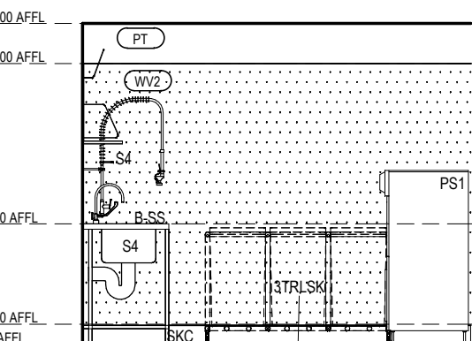
RACF BOH - SLUICE ELEVATION 2 Scale 1: 50
