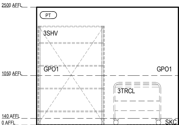
RACF BOH - CLEANER - TYPE 2 ELEVATION 1 Scale 1: 50
