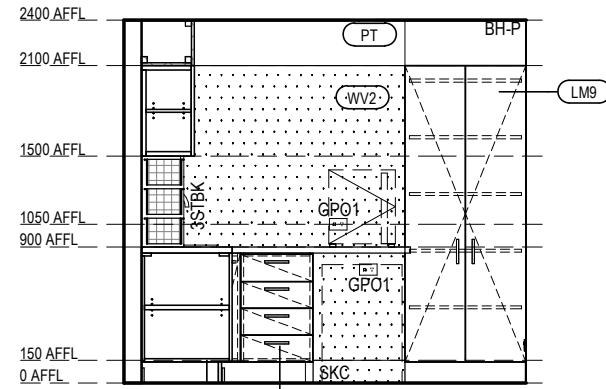
RACF BOH - TREATMENT ELEVATION 3 Scale 1: 50
