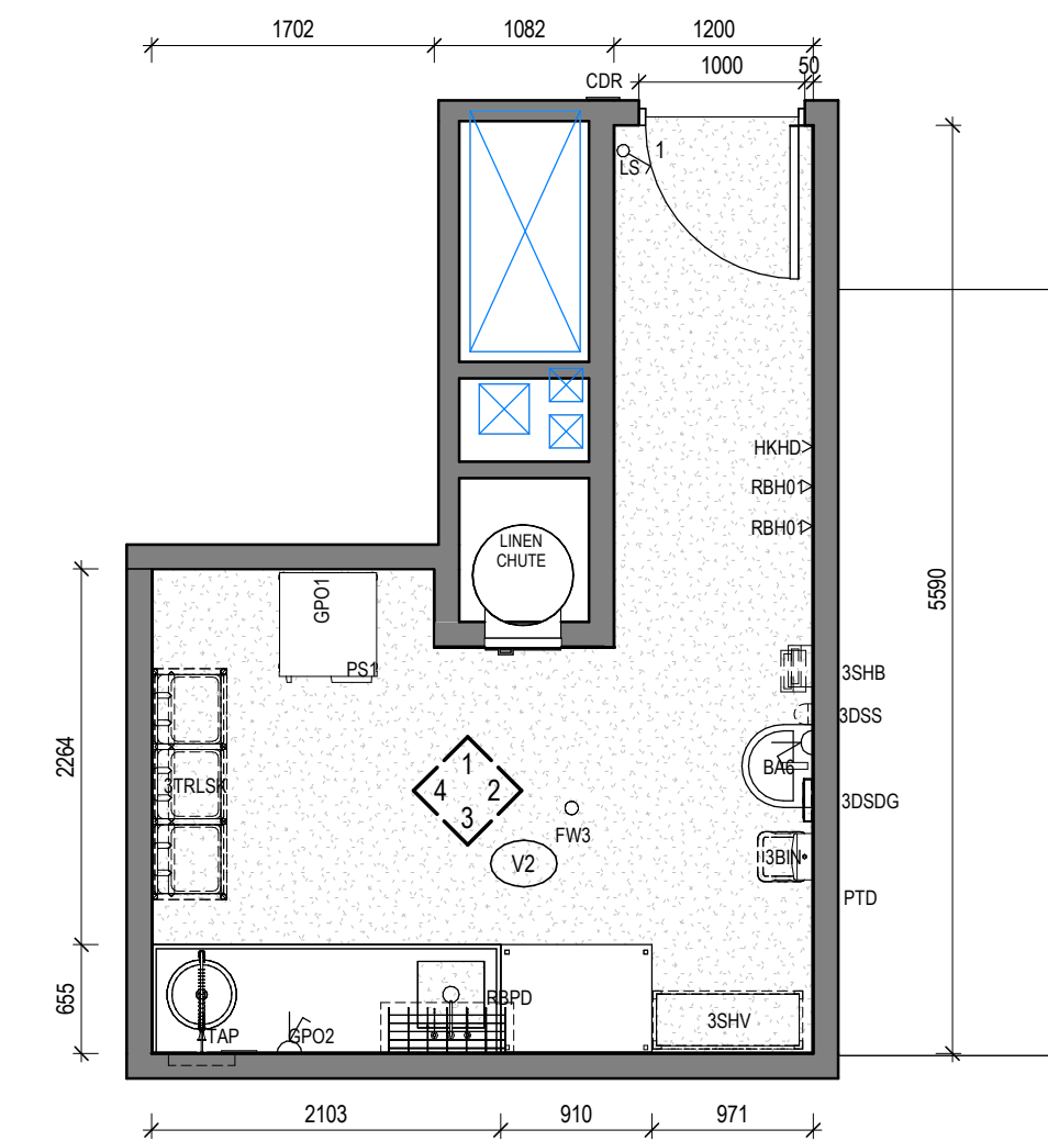
7 RACF-SLUICE Scale 1: 50
