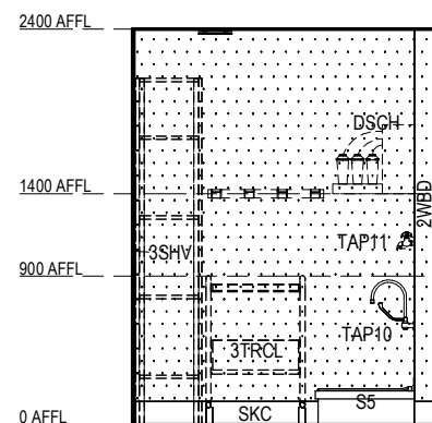
RACF BOH - CLEANER - TYPE 1 ELEVATION 3 Scale 1: 50
