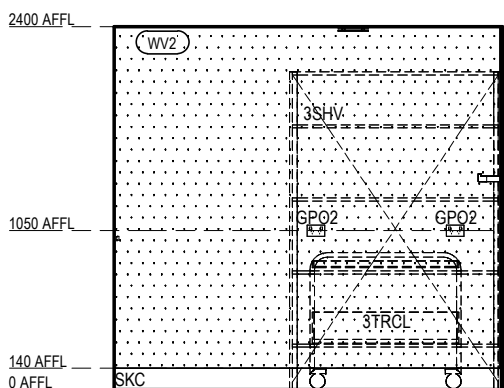
RACF BOH - CLEANER - TYPE 1 ELEVATION 2 Scale 1: 50
