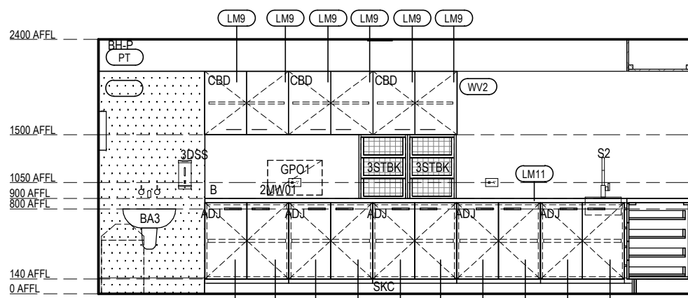
RACF BOH - TREATMENT ELEVATION 2 Scale 1: 50
