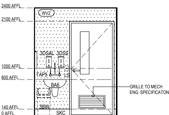
RACF BOH - CLEANER - TYPE 1 ELEVATION 1 Scale 1: 50
