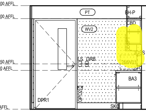
RACF BOH - TREATMENT ELEVATION 1 Scale 1: 50
