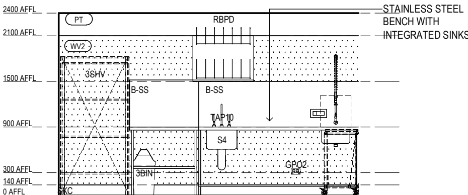
RACF BOH - SLUICE ELEVATION 3 Scale 1: 50
