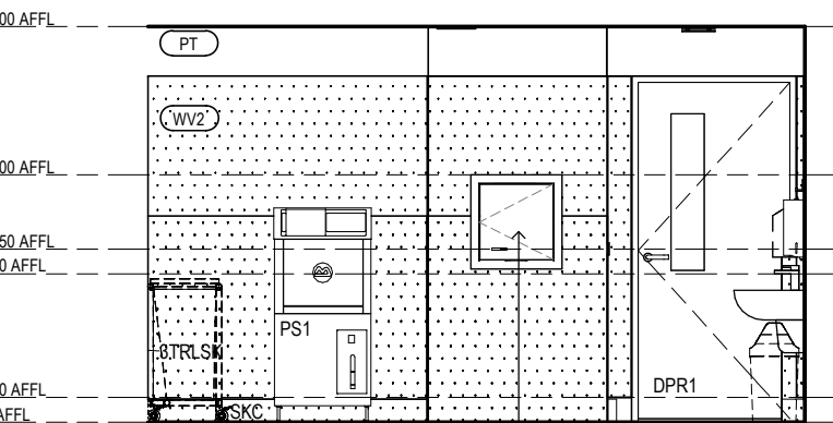
RACF BOH - SLUICE ELEVATION 1 Scale 1: 50
