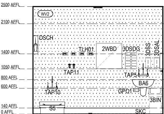
RACF BOH - CLEANER - TYPE 2 ELEVATION 3 Scale 1: 50
