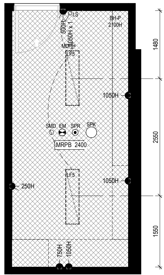
6 RCP-TREATMENT Scale 1: 50
