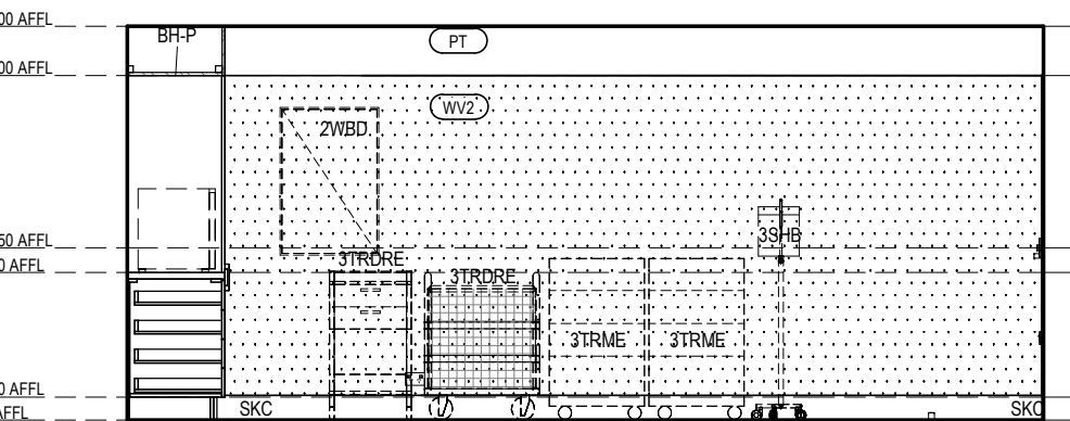
RACF BOH - TREATMENT ELEVATION 4 Scale 1: 50
